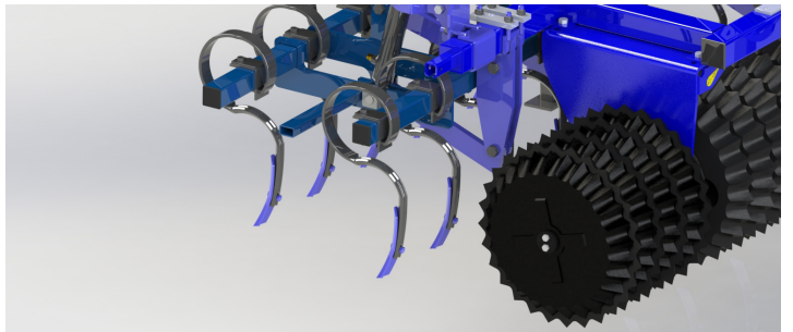
FrontFlex fitted with 2 rows of H/D 45 x 10mm spring tines.
